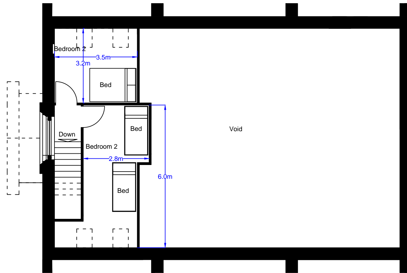
8DT16: 8 Derby Terrace 1st Floor as Proposed Page 1 of 1, Scale 1:100 at A3
